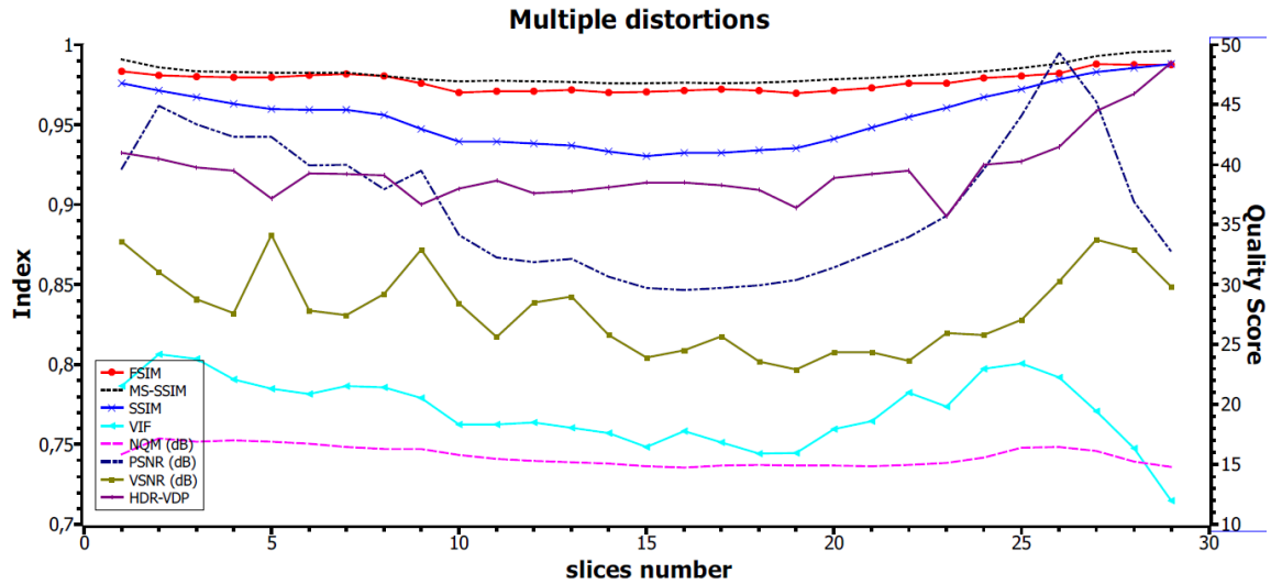
Figure 9. Multiple distortions applied on the volume A with a rotation of 0.1^\circ , a grayscale modification of 0.8 and a Gaussian noise of 15% of the maximum value of each slice
