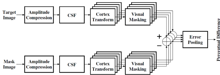
Figure 3. Data flow diagram of the Visual Differences Predictor (VDP) 19
