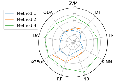
(b) F1-Score
