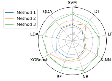
(a) Accuracy
